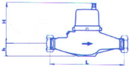
Flowmeter ½" to 1-½"
